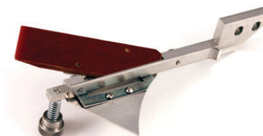
SCRAPER SUPPORT BRACKET ASSEMBLY M4-468/A | Ref: 44468
