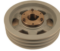
REAR DRIVE PULLEY & BUSHING NP2-PLY2 | Ref: N/A
