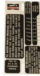
PRESSURE INDICATING NAME PLATE (TONNAGE) SD4-28 | Ref: N/A
