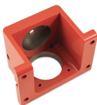
LEFT SIDE TABLET THICKNESS SERVO BRACKET NP5-568-B1 | Ref: N/A
